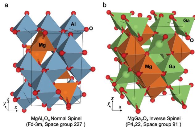
Fig. 36 Normal and inverse spinel structures. (a) MgAl 2 O 4 normal and (b) MgGa 2 O 4 inverse ground state atomic configurations. In each case the unit cell is shown by solid black lines. Octahedral and tetrahedral atomic coordination environments are also identified by the coordination polyhedra in each case. Reproduced with permission from ref. 717. Copyright Nature Publishing 2020.
