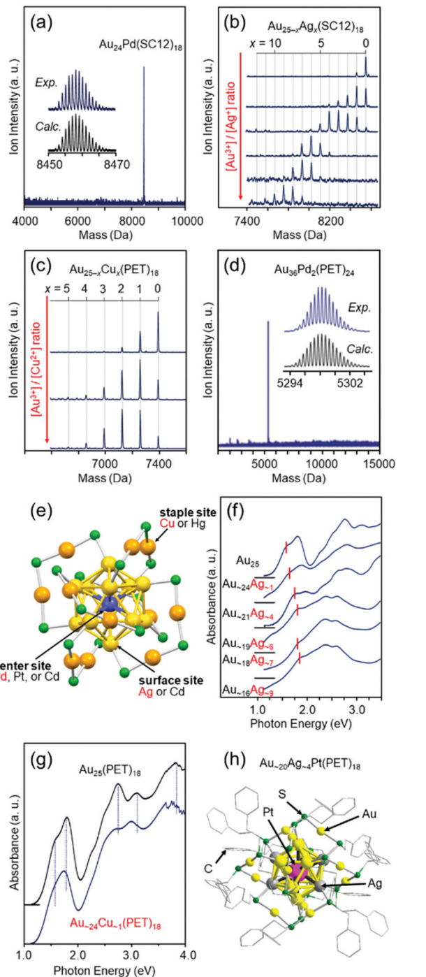
Fig. 6 Negative-ion MALDI mass spectra of (a) Au 24 Pd(SC12) 18 , 110 (b) Au 25-x Ag x (SC12) 18 , 111 and (c) Au 25-x Cu x (PET) 18 , 112 (d) Negative-ion ESI mass spectrum of Au 36 Pd 2 (PET) 24 . 114 (e) Preferential substitution site in Au 25 (SR) 18 for each element. 116 Blue, yellow, and orange spheres represent Au atoms, and green spheres represent S atoms. The R groups are omitted for clarity. Optical absorption spectra of (f) [Au 25-x Ag x (SC12) 18 ] - and (g) [Au ~24 Cu ~1 (PET) 18 ] - . 112,158 (h) Geometric structure of [Au ~20 Ag ~4 Pt(PET) 18 ] 0 . 117 Reproduced with permission from ref. 110-112, 114, 116 and 117. Copyright 2010 The Royal Society of Chemistry, 2012 American Chemical Society, 2012 The Royal Society of Chemistry, 2016 The Royal Society of Chemistry, and 2018 American Chemical Society.
