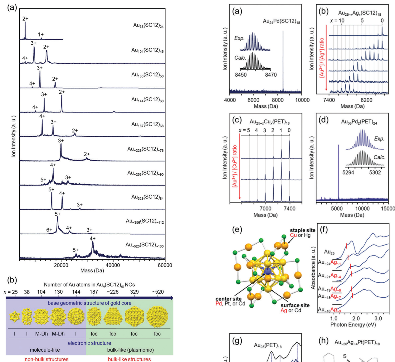
Fig. 5 (a) Positive-ion ESI mass spectra of Au n (SC12) m NCs. (b) Non-bulk to bulk transition between Au 144 (SC12) 60 and Au 187 (SC12) 68 in the Au n (SC12) m -NC system. 109 Reproduced with permission from ref. 109. Copyright 2015 American Chemical Society.
