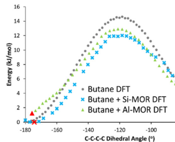
Fig. 4 DFT calculated energy of rotation about the \text{C-C-C-C} dihedral angle in n -butane, transitioning from the antiperiplanar ( -180^\circ ) to the gauche conformer ( -60^\circ ) for butane when unconfined (Butane DFT), in siliceous mordenite (Butane + Si-MOR DFT) and acidic Al-substituted mordenite (Butane + Al-MOR DFT). Red symbols represent minima, as confirmed by frequency calculations, as shown in Fig. 3 and Fig. S15 (ESI † ). Final Gauche conformers (Fig. S16, ESI † ) were determined based on the progression of \text{C-C-C-C} dihedral angle in the optimisation sequence.
