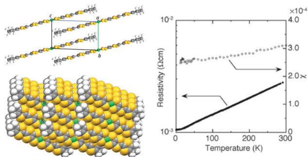
Fig. 4 Left: Details showing the domino-like molecular overlapping and the 3D compact molecular packing in the crystal structure [Ni(tmtd) 2 ]. Right: Temperature dependence of resistivity and magnetic susceptibility ( \chi , emu mol -1 ) of [Ni(tmtd) 2 ]. From Tanaka, H., Okano, Y., Kobayashi, H., Suzuki, W., & Kobayashi, A. (2001). A Three-Dimensional Synthetic Metallic Crystal Composed of Single-Component Molecules. Science , 291(5502), 285–287. DOI: 10.1126/science.291.5502.285. Reprinted with permission from AAAS.
