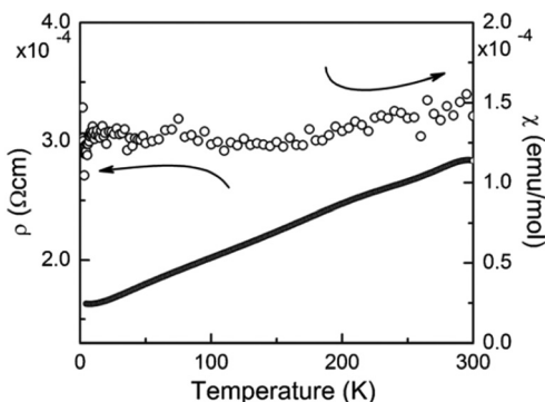
Fig. 5 Temperature dependence of resistivity ( \rho ) and magnetic susceptibility ( \chi ) of [Pt(tmtd) 2 ] measured in a compressed polycrystalline sample. Reprinted with permission from ref. 41. Copyright©2009 Wiley-VCH Verlag GmbH & Co. KGaA, Weinheim.
