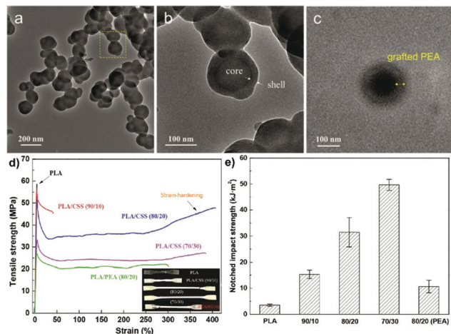
Fig. 7 (a–c) TEM images of SNP- g -PEA core-shell NPs, (d) stress-strain curves of PLA and PLA/SNP- g -PEA core-shell NP composite (inset shows optical photo of the samples), (e) notched impact strengths of PLA and PLA/SNP- g -PEA core-shell NP composite. (Reproduced with permission from ref. 153. Copyright American Chemical Society, 2018.)
