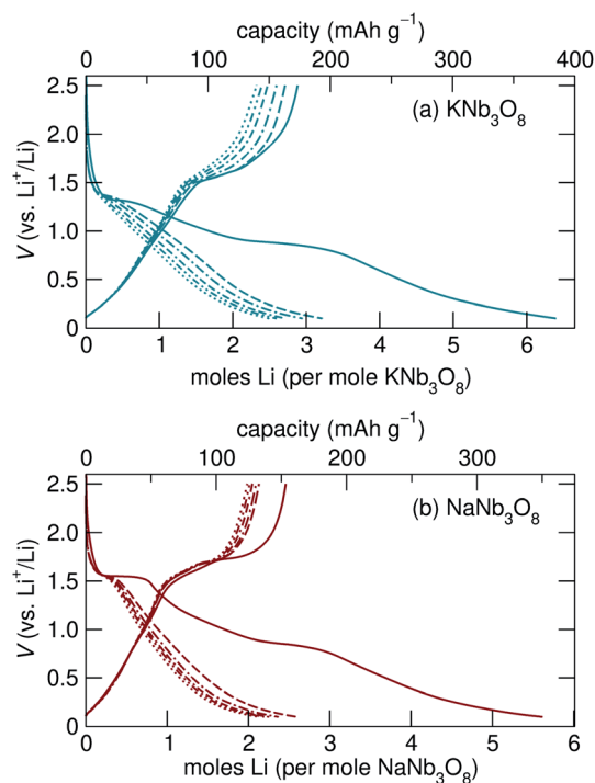
Fig. 6 Galvanostatic cycling of (a) \text{KNb}_3\text{O}_8 and (b) \text{NaNb}_3\text{O}_8 , with the first cycle in solid lines and increasingly broken lines for subsequent cycles. In their first cycle, \text{KNb}_3\text{O}_8 and \text{NaNb}_3\text{O}_8 have similar cycling profiles, consisting of a combination of plateaued and sloped regions, with asymmetry in the profiles between discharge and charge. Later cycling shows a slow fade in capacity for both compounds.
