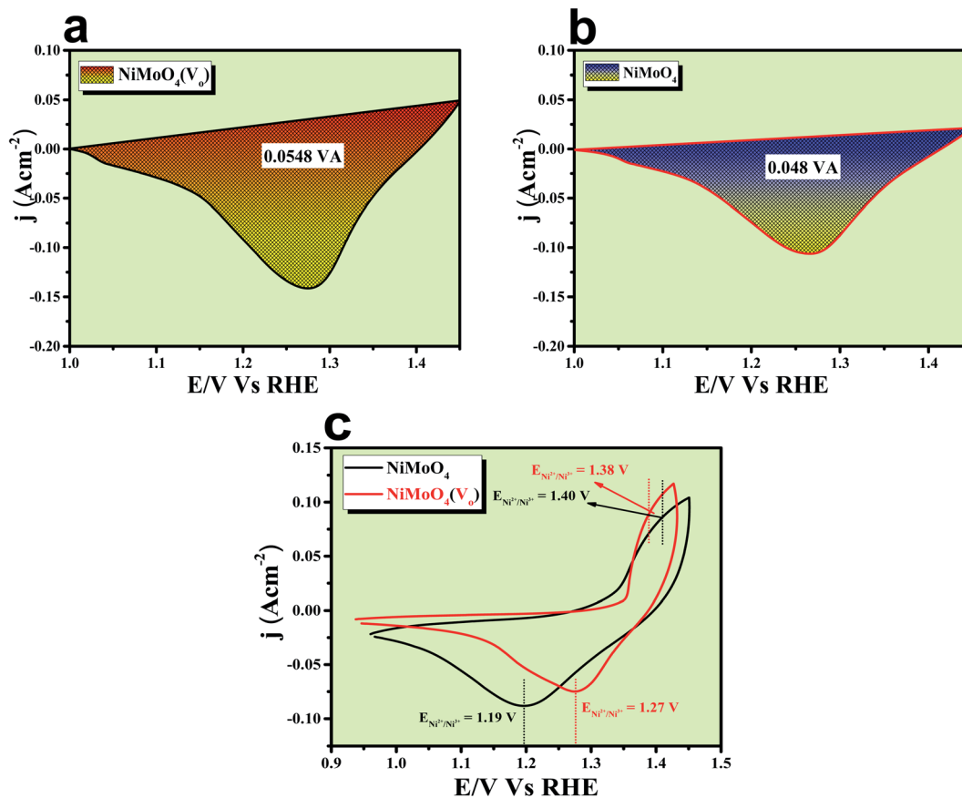
Fig. 11 (a) and (b) Reduction peak area of rod-like \text{NiMoO}_4(\text{V}_\text{o}) and \text{NiMoO}_4 ; (c) CV cycles for \text{NiMoO}_4(\text{V}_\text{o}) and \text{NiMoO}_4 .
