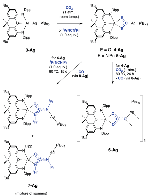
Scheme 3 Reactions of silver–aluminium compound 3-Ag with CO 2 and 1 PrNCN i Pr.
