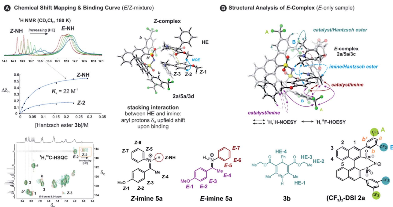
Fig. 2 Chemical shift mapping and NOE/HOE analysis proves bifunctional binding in the ternary complex: (A) stronger binding of Z -imine from chemical shift mapping; NMR titration of (CF 3 ) 2 -DSI 2a/5a E/Z mixture (20 mM) with 0–15 eq. Hantzsch ester 3b , followed by ^1\text{H} NMR and ^1\text{H},^{13}\text{C} -HSQC spectra in \text{CD}_2\text{Cl}_2 at 180 K (NH signals split into doublets by ^1J_{\text{NH}} due to the iminium ^{15}\text{N} nucleus). Fitting of the \Delta\delta_{\text{H}} ( Z -NH and Z -2) gave a binding constant K_a = 22 \text{ M}^{-1} for Z -5a. The plausible calculated structure 2a/5a/3d (TPSS-D3(BJ)/def2-SVP/SMD( \text{CH}_2\text{Cl}_2 )) shows the NOE contact and explains the most pronounced chemical shift differences for Z -2/ Z -3 resonances upon binding. (B) A plausible calculated structure of ternary of E -complex 2a/5a with Hantzsch ester 3c with key NOE and HOE contacts shown.
