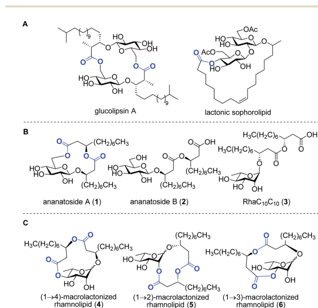
Fig. 1 Examples of macrodilactone-containing glucolipids produced by microbes (A); structures of target ananatoside A ( 1 ) and ananatoside B ( 2 ) produced by Pantoea ananatis along with the related RhaC 10 C 10 ( 3 ) (B); structures of target macrodilactone-containing rhamnolipids 4–6 (C). Lactone functionalities are highlighted in blue.
