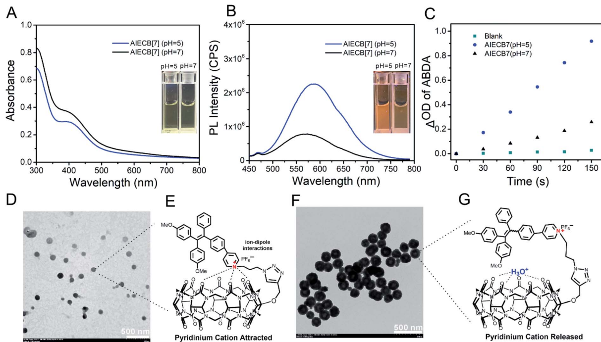
Fig. 1 UV-vis absorbance (A) and fluorescence spectra (B) of AIECB[7] assemblies. The inset images were taken under white light (A) and 365 nm UV light (B), respectively. (C) Singlet oxygen ( 1 O 2 ) generation of AIECB[7] determined by measuring the absorbance changes of ABDA at 378 nm. Typical TEM images and postulated configurations of AIECB[7] assemblies in aqueous solutions at pH = 7 (D and E) and pH = 5 (F and G), respectively. Scale bars: 500 nm.
