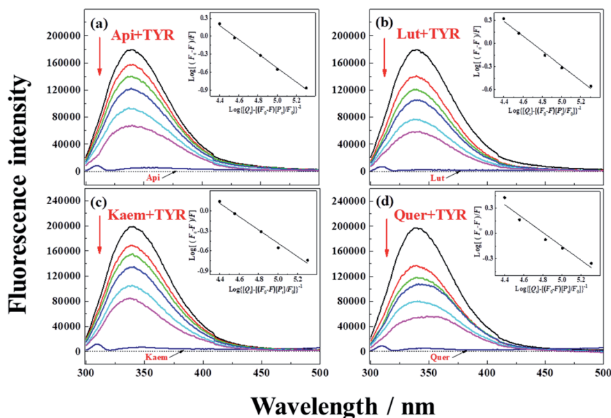
Fig. 2 Fluorescence emission spectra of 28 μg mL -1 tyrosinase in the presence of varying concentrations, 0, 5, 10, 15, 28, 40 μM (a) Api, (b) Lut, (c) Kaem and (d) Quer at 25 °C, respectively. \lambda_{\text{ex}} = 280 nm. Insets: plots of \log((F_0 - F)/F) at \lambda_{\text{em}} = 340 nm according to the double-logarithm eqn (3). F_0 and F represent fluorescence intensities of solutions in the absence and presence of flavonoids.
