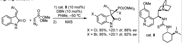
Scheme 3 1,3-Dipolar cycloaddition followed by ring contraction to 3,3'-cyclopropyl spirooxindoles.
