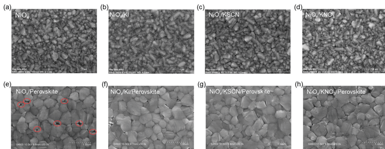
Fig. 1 SEM images of (a) \text{NiO}_x HTLs and (b) KI, (c) KSCN and (d) \text{KNO}_3 modified \text{NiO}_x HTLs. SEM images of perovskite layers grown on (e) \text{NiO}_x HTL, (f) \text{NiO}_x /KI HTL, (g) \text{NiO}_x /KSCN HTL and (h) \text{NiO}_x /KNO 3 HTL.
