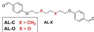
Fig. 3 Molecular structure of the tuneable dialdehyde monomer, for which X is either CH 2 (AL-C, apolar chain) or O (AL-O, polar chain).
