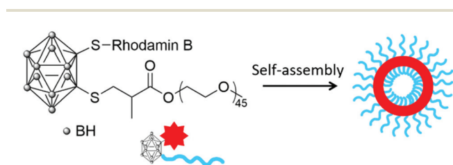
Scheme 2 Self-assembly into vesicles of a fluorescent carborane-conjugated POEGMA.
