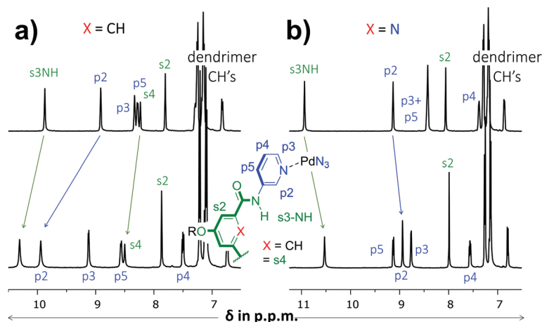
Fig. 2 Partial ^1\text{H} NMR spectra involving dipyrilidyl ligands 1 (a) and 2 (b). The top spectra are of pure ligand and the bottom spectra are of the [\text{Pd}_2(\text{Ligand})_4]\text{BF}_4 complexes. The solvent is \text{CD}_2\text{Cl}_2 containing 5% \text{dmsO}-d_6 and further details are given in the ESI.†
