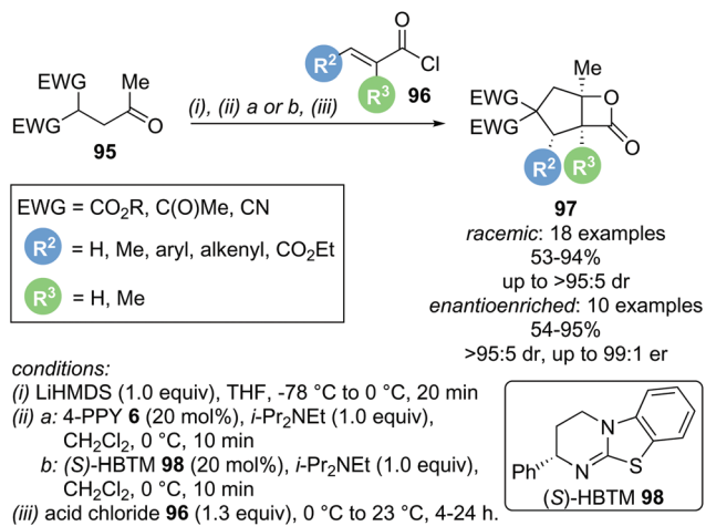
Scheme 20 Michael-aldol-lactonization cascade.
