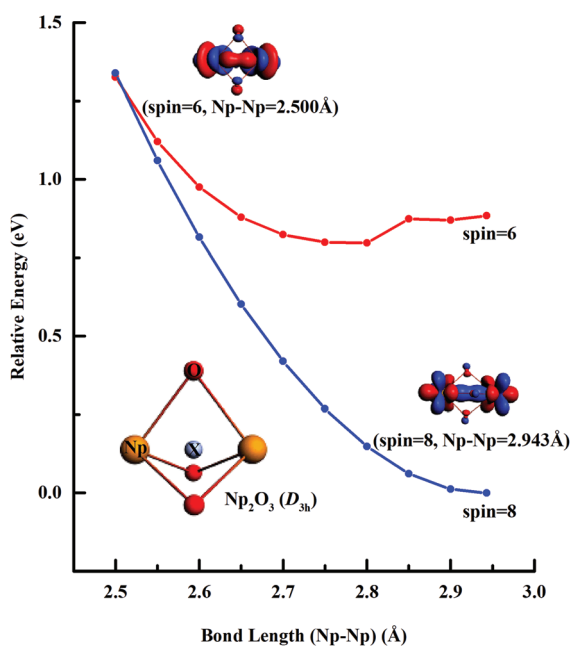
Fig. 3 Linear transit (LT) potential energy curves of \text{Np}_2\text{O}_3 calculated at the SR-DFT/PBE level.
