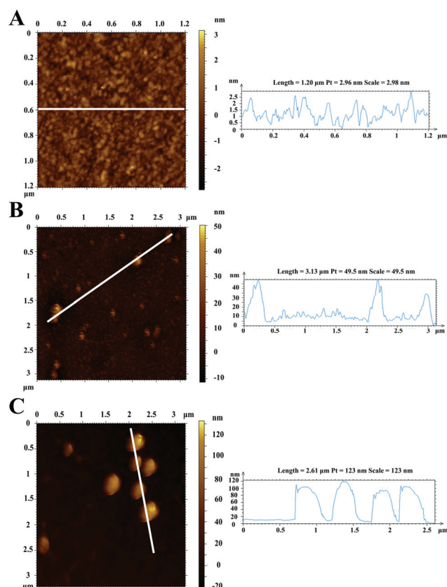
Fig. 4 2D AFM images and line profiles of the bare gold chip (A), GNC- and protein-functionalized gold film (B), and the MNPs-Ab modified gold surface (C).
