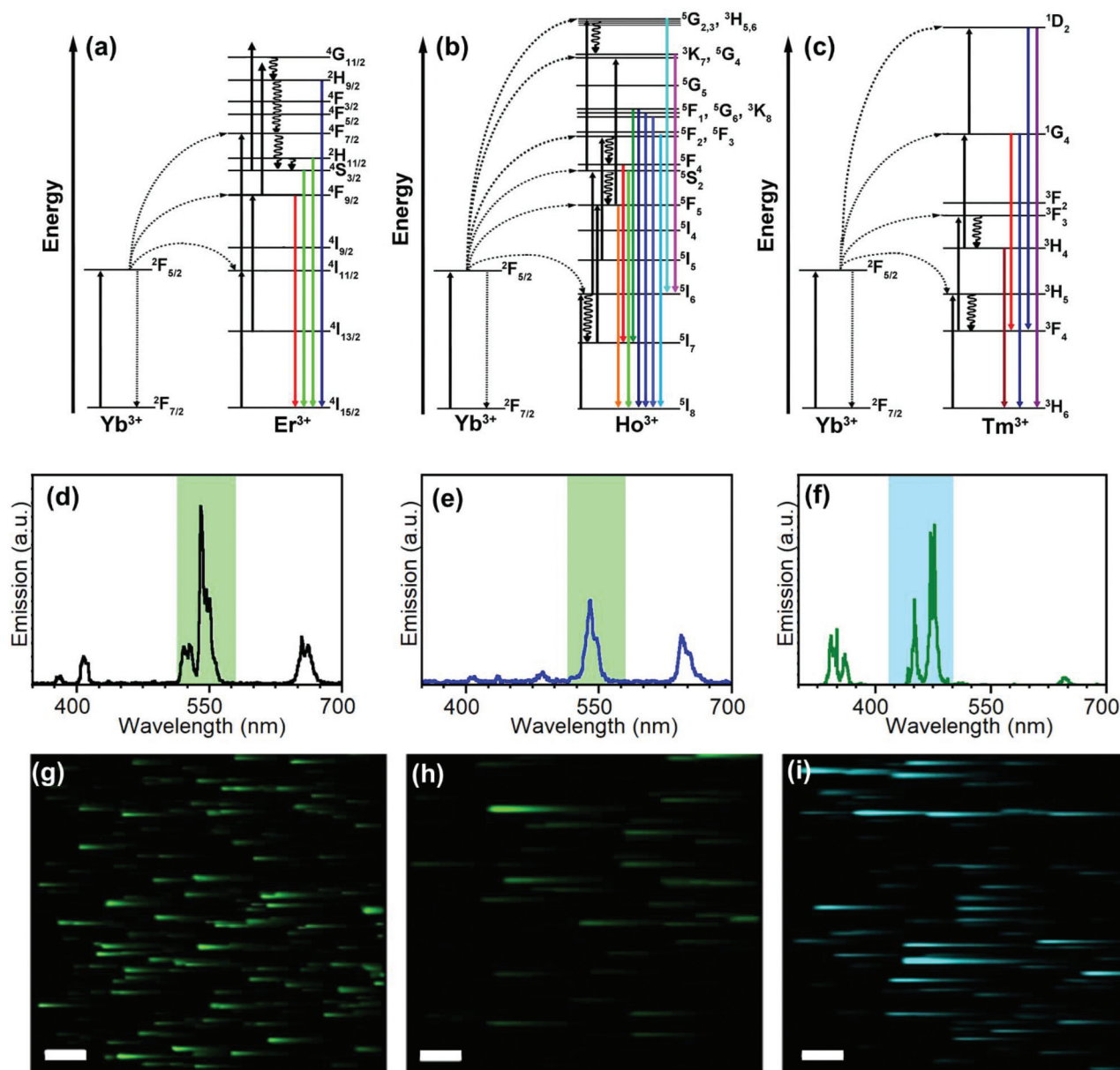
Fig. 1 Analysis of the UCNP emissive properties. (a–c) Energy transfer processes involved in the emission of UC_{Er} (a), UC_{Ho} (b) and UC_{Tm} (c). (d–f) Luminescence emission spectra of colloidal UCNP (1 mg mL -1 ) in toluene (d) UC_{Er,2} , (e) UC_{Ho} and (f) UC_{Tm} ( \lambda_{exc} = 975 nm; I = 93 W cm -2 ). The colored columns indicate the detection channel range (C1, blue: 420–500 nm; C2, green: 515–580 nm) which was used to register the corresponding (g–i) NIR-LSM images ( \lambda_{exc} = 975 nm and F_d = 0.2 J cm -2 ). Scale bar: 50 \mu m.
