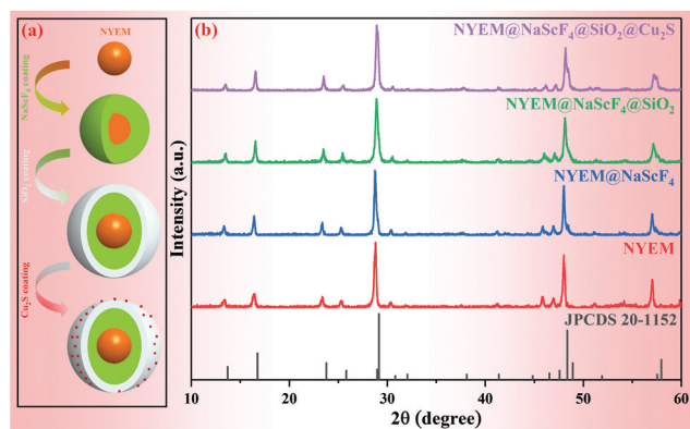
Fig. 1 (a) A description of the preparation of \text{NYEM}@/\text{NaScF}_4@/\text{SiO}_2@/\text{Cu}_2\text{S} . (b) XRD diffraction patterns of the samples synthesized at various steps along with the reference data of hexagonal \text{NaScF}_4 (JCPDS 20-1152).
