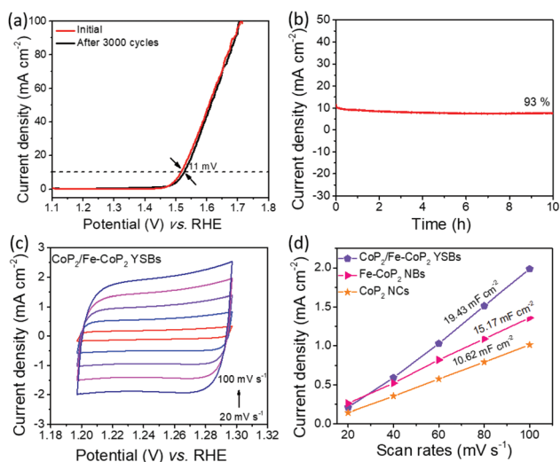
Fig. 8 (a) LSV curves of CoP 2 /Fe-CoP 2 YSBs before and after 3000 cycles. (b) Chronoamperometry stability test at a static potential of 1.50 V (vs. RHE) for 10 hours. (c) Cyclic voltammery curves of CoP 2 /Fe-CoP 2 YSBs at different scan rates. (d) The capacitive current density as a function of scan rate for CoP 2 /Fe-CoP 2 YSBs, Fe-CoP 2 NBs and CoP 2 NCs. The measured double-layer capacitance of the system is taken as the average of the absolute value of the slope of linear fits to the data.
