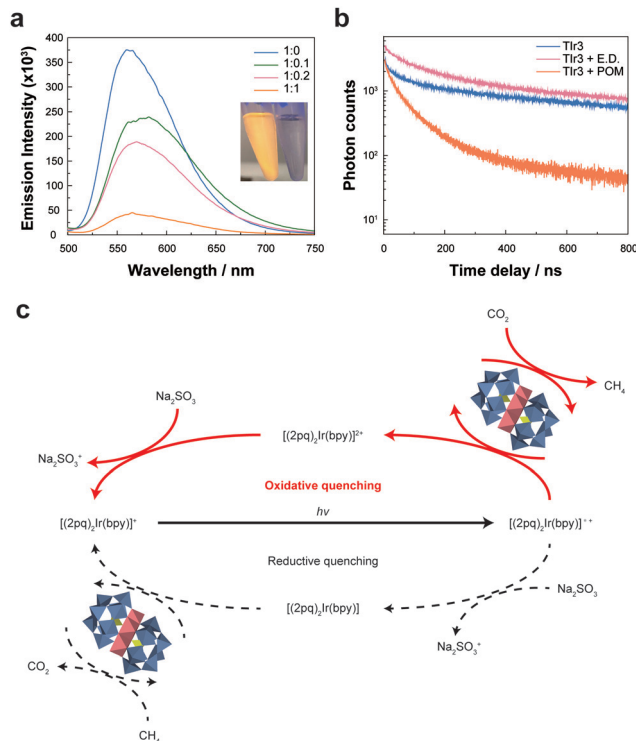
Fig. 3 Photophysical analysis of photocatalytic CO_2RR systems. (a) Static photoluminescence spectra of TlR3 (50 \mu\text{M} ) without (blue line) and with ZnPOM at different concentration ratios of TlR3 and ZnPOM. The inset shows a photograph of TlR3 solutions under UV light without (left) and with (right) ZnPOM (50 \mu\text{M} ). (b) Time-correlated single-photon counting for lifetime measurements of TlR3 without and with POM or sacrificial electron donor (E.D.) Na_2SO_3 . (c) A suggested mechanistic pathway for the photocatalytic CO_2RR to CH_4 using ZnPOM and TlR3.
