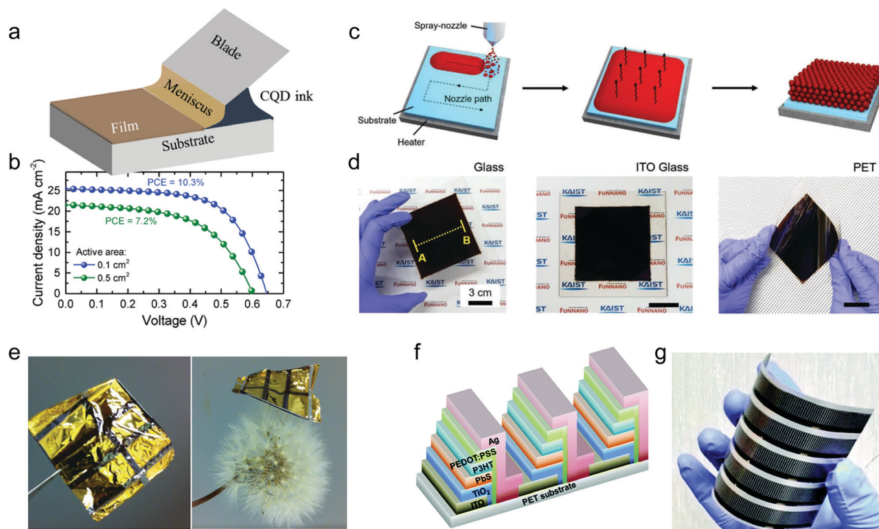
Fig. 6 (a) Schematic of the employed blade-coating setup. (b) J–V curves of 0.1 \text{ cm}^2 (blue) and 0.5 \text{ cm}^2 (green) active area blade-coated solar cells. Reprinted with permission from ref. 69. Copyright 2018, Wiley-VCH. (c) Scheme of the fabrication process of CQD films by using the spray-coating method. (d) Photograph of CQD films ( 10 \text{ cm} \times 10 \text{ cm} ) on a glass substrate, indium tin oxide (ITO) glass substrate, and polyethylene terephthalate (PET) substrate. Reprinted with permission from ref. 110. Copyright 2019, Wiley-VCH. (e) Photograph of the flexible PbS CQD solar cell. The size of the flexible substrate with six solar cells is \sim 2 \times 2 \text{ cm}^2 . The flexible solar cell is placed on a dandelion without any deformation of the dandelion, illustrating its extremely lightweight feature. Reprinted with permission from ref. 112. Copyright 2018, The Royal Society of Chemistry. (f) Schematic diagram of the serial connection of PbS CQD solar cells. (g) Photograph of the PbS CQD solar modules on the flexible PET film with an active area of 30 \text{ cm}^2 , which was fabricated employing R2R printing. Reprinted with permission from ref. 113. Copyright 2015, The Royal Society of Chemistry.
