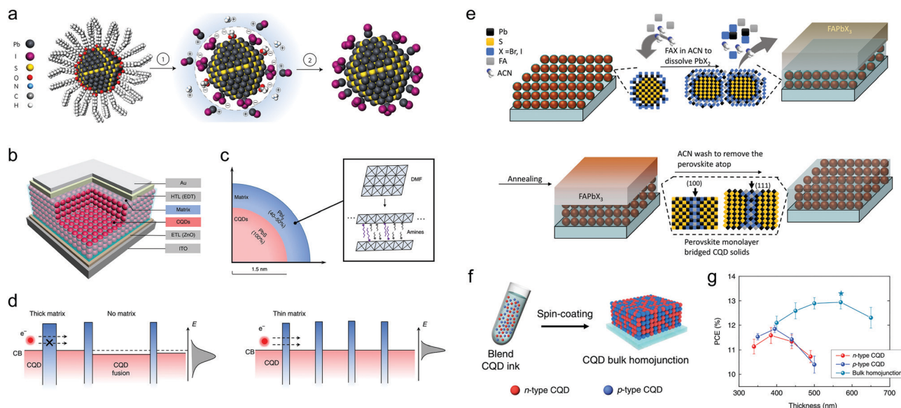
Fig. 3 (a) Solution-phase ligand exchange with metal halide precursors and ammonium acetate. Process 1 (ligand exchange): the bulky oleic acid ligands are replaced by the [PbX_3]^- anions with the aid of ammonium protons. The CQD surface is stabilized by both [PbX_3]^+ and [NH_4]^+ . Process 2 (CQD precipitation): after ligand exchange, CQDs are precipitated via the addition of toluene, an anti-solvent, and are separated by centrifugation. Reprinted with permission from ref. 17. Copyright 2017, Nature Publishing Group. (b) Schematic diagram of the effective medium model of the CQD absorber in a solar cell, where CQDs (red) assemble in a matrix medium (blue). (c) The matrix consists of PbI_2 , which is enough to account for the formation of full monolayer coverage on the surfaces of PbS CQDs (bandgap \sim 1.3 eV and diameter \sim 3 nm). The dimensional structure of the matrix can be tuned using solvents. (d) The schematic diagram for the effect of the matrix on the structural and energetic order of CQD film. Confining the matrix dimensionality between the CQDs and improving its homogeneity throughout the film can increase the photocarrier diffusion length and reduces the V_{oc} deficit. Reprinted with permission from ref. 43. Copyright 2018, Nature Publishing Group. (e) Schematic of the formation of monolayer perovskite bridges among the QDs. The perovskite matrix is formed first by soaking the pre-exchanged CQD films in a FAX ( X = Br, I ) solution, where the FAX solution dissolves the PbX_3^- ligands and perovskite grows between adjacent PbS CQDs. The films are annealed and then washed with acetonitrile to remove excess perovskite. Reprinted with permission from ref. 18. Copyright 2014, Elsevier. (f) The bulk-homojunction films were fabricated by depositing the blended CQD inks comprising n-type and p-type CQDs. (g) Thickness-dependent PCE for bulk-homojunction devices and n-type CQD devices. Bulk-homojunction devices enable the use of much thicker CQD films compared with the case of n-type CQD devices, indicating the increase of carrier diffusion length. Reprinted with permission from ref. 49. Copyright 2020, Nature Publishing Group.
