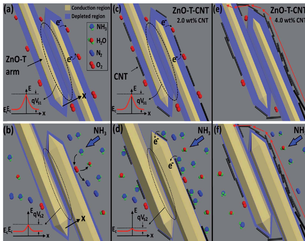
Fig. 10 Illustration of sensor in air (a) ZnO-T, (c) ZnO-T-2 wt% CNT networks and (e) ZnO-T-4 wt% CNT networks and in NH 3 atmosphere (b) ZnO-T, (d) ZnO-T-2 wt% CNT networks and (f) ZnO-T-4 wt% CNT networks 155 (reprinted with permission from ref. 155. Copyright (2017) American Chemical Society).
