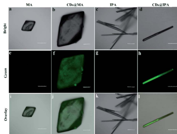
Fig. 2 Fluorescence confocal microscopic images of (a, e and i) MA, (b, f and j) CDs@MA, (c, g and k) IPA and (d, h and l) CDs@IPA crystals. The green channel was collected in the range of 520–560 nm ( \lambda_{\text{ex}} = 405 nm). Scale bar: 100 \mu\text{m} .
