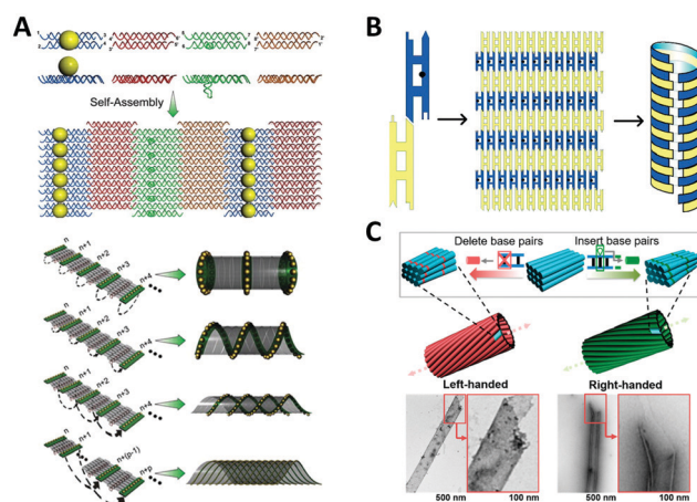
Fig. 5 Chiral arrangement of metal NPs assisted by scaffold-free DNA tiles. (A) Schematic of the formation of AuNPs helix by four different tiles. 112 Reproduced from ref. 112 with permission from the AAAS. (B) The DNA tube with structural chirality comprising two kinds of tiles. 114 Reproduced from ref. 114 with permission from the American Chemical Society. (C) The large helical tubes designed by SST. 115 Reproduced from ref. 115 with permission from the American Chemical Society.
