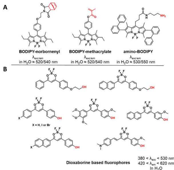
Fig. 5 Examples of difluoroboron complexes used for BCP labeling: (A) BODIPY derivatives and (B) dioxaborine based fluorophores.
