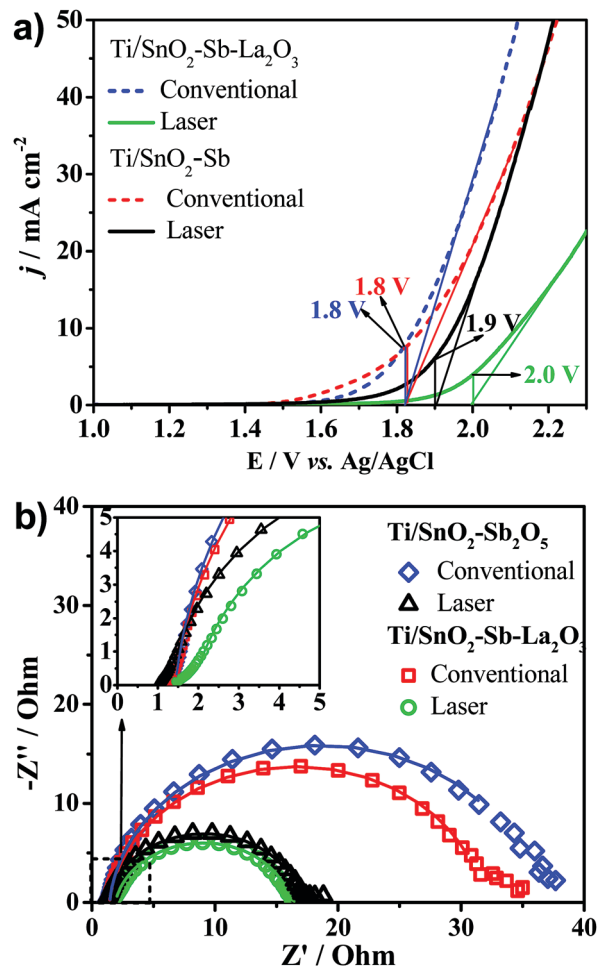
Fig. 6 Linear sweep voltammetry profiles recorded at a scan rate of 10 \text{ mV s}^{-1} (a) and Nyquist plots of the anodes (b) taken at the OER onset potential from 0.1 to 10^4 Hz (inset is the expanded view of the high-frequency region). Electrolyte: 0.5 \text{ mol L}^{-1} \text{ H}_2\text{SO}_4 .
