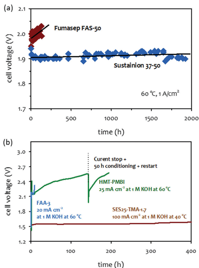
Fig. 11 (a) 1 M KOH-fed AEMWEs at 60\text{ }^{\circ}\text{C} at a current density of 1\text{ A cm}^{-2} . 131 AEM: Fumasep ® FAS-50 (50 \mu\text{m} thick) or Sustainion ® 37–50 (50 \mu\text{m} thick), ionomer: Nafion, anode: NiFe 2 O 4 ( 2\text{ mg cm}^{-2} ); cathode: NiFeCo ( 2\text{ mg cm}^{-2} ). The durability was measured at 60\text{ }^{\circ}\text{C} under ambient pressure. Reproduced with permission. 131 Copyright 2017, Elsevier. (b) Short-term test of 1 M KOH-fed AEMWEs employing alkaline-stable AEMs. AEM/ionomer: HMT-PBI (43 \mu\text{m} thick)/HMT-PBI, Fumatech FAA-3 (50 \mu\text{m} thick)/FAA-3, anode and catalysts: Pt/C (0.5 \text{mg}_{\text{Pt}}\text{ cm}^{-2} ), AEM/ionomer: SES25-TMA-1.7 (53 \mu\text{m} thick)/FLN-55, anode: IrO 2 ( 1\text{ mg cm}^{-2} ); cathode: PtRu/C (50 wt% Pt, 25 wt% Ru, 0.5\text{ mg}_{\text{Pt}}\text{ cm}^{-2} ). Reproduced with permission. 18 Copyright 2016, Royal Society of Chemistry.
