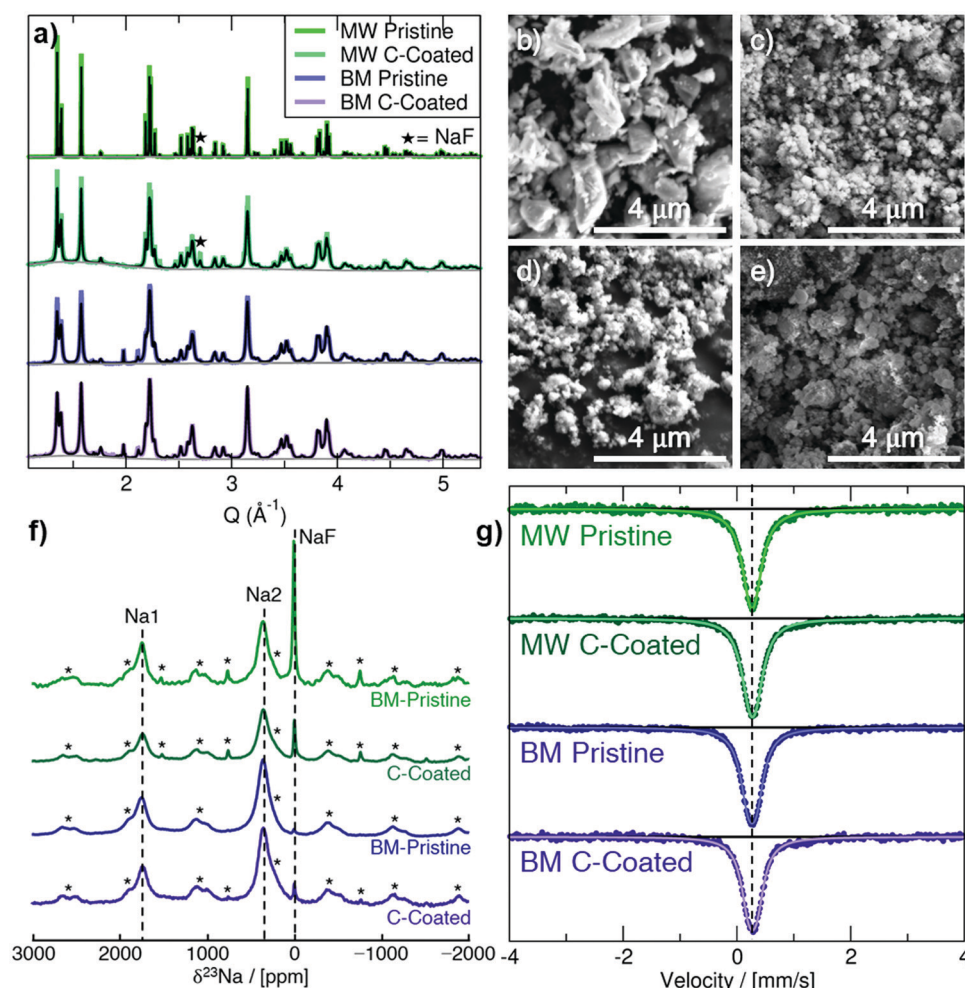
Fig. 1 Structural characterization of as-prepared Na 3 FeF 6 materials. (a) SXRD pattern and Rietveld refinement (black) for each sample. (b–e) SEM images obtained of MW pristine (b), MW C-coated (c), BM pristine (d), and BM C-coated (e) samples. (f) 23 Na spin echo NMR spectra collected on the as-prepared materials. Each spectrum is scaled according to the number of moles of material in the rotor and the number of scans collected during the experiment. Spinning sidebands are indicated by an asterisk (*). (g) Zero-field, 298 K 57 Fe Mössbauer spectra obtained on the as-prepared materials. The dashed line corresponds to an isomer shift (δ) of 0.27 mm s -1 typical of an Fe 3+ ion in an octahedral environment.
