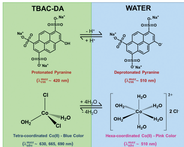
Fig. 3 Structures of various forms of pyranine and Co II based on the solubilizing media.
