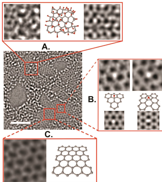
Fig. 6 Aberration-corrected TEM image of a single sheet of suspended GO. The scale bar is 2 nm. Expansion (a) shows, from left to right, a 1 nm 2 enlarged oxidized region of the material, then a proposed possible atomic structure of this region with carbon atoms in gray and oxygen atoms in red, and finally the average of a simulated TEM image of the proposed structure and a simulated TEM image of another structure where the position of oxidative functionalities has been changed. Expansion (b) focuses on the white spot on the graphitic region but stayed stationary for 3 frames (6 seconds) at a hydroxyl position (left portion of expansion (b)) and for 7 frames (14 seconds) at a (1,2) epoxy position (right portion of expansion (b)). The ball-and-stick figures below the microscopy images represent the proposed atomic structure for such functionalities. Expansion (c) shows a 1 nm 2 graphitic portion from the exit plane wave reconstruction of a focal series of GO and the atomic structure of this region. Reproduced from ref. 17 with permission from Wiley-VCH.
