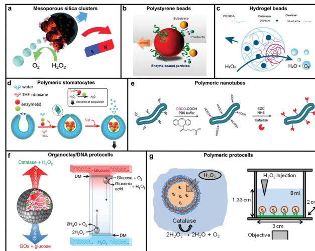
Fig. 4 Designs for catalase powered MNMs. (a) Mesoporous silica nanoclusters with magnetic control bound to catalase on one side, 121 (b) polystyrene beads coated with catalase by biotin–streptavidin linkage, 69 (c) biocompatible hydrogel fabricated by PEGDA and dextran, 124 (d) polymeric (PEG- b -PS) stomatocytes encapsulated with enzymes, 124 (e) biodegradable polymeric (PEG- b -PDLLA) nanotubes coated with catalase, 125 (f) organoclay/DNA protocells encapsulated with enzymes, 126 and (g) polymeric protocells encapsulated with catalase for autonomous motion. 127 Adapted with permission from ref. 121 and 125. Copyrights 2015, 2018 Royal Society of Chemistry. Adapted with permission from ref. 69 and 115. Copyrights 2015 and 2016 American Chemical Society. Adapted with permission from ref. 124 and 127. Copyrights 2018 Wiley. Adapted with permission from ref. 126. Copyrights 2018 Springer Nature.
