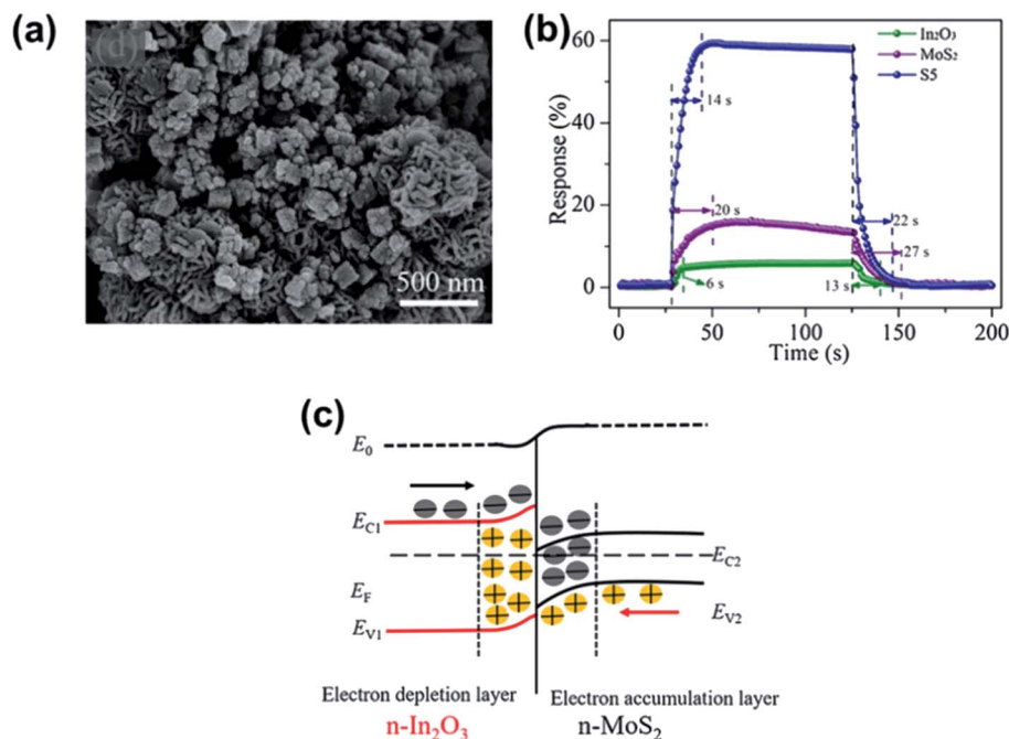
Fig. 21 (a) SEM images of In 2 O 3 nanocubes/flower-like MoS 2 hybrids. (b) The response and recovery characteristics of In 2 O 3 , MoS 2 and In 2 O 3 /MoS 2 (S5) film sensors exposed to 50 ppm HCHO gas. (c) The energy band diagram for the n-n junction of the In 2 O 3 /MoS 2 film. Reprinted with permission from ref. 167. Copyright 2018, Elsevier.
