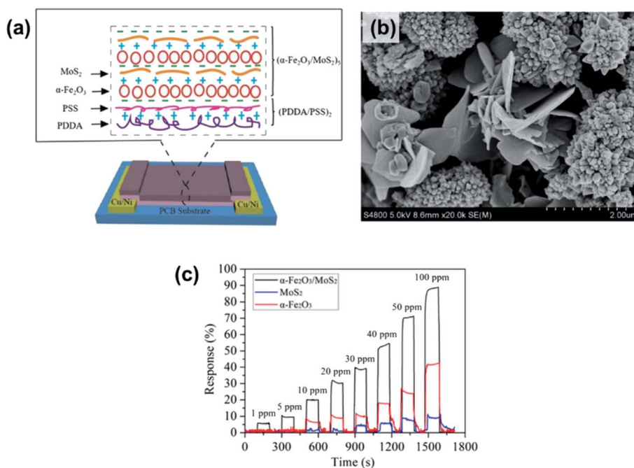
Fig. 22 (a) Schematic of an \alpha -Fe 2 O 3 /MoS 2 gas sensor. (b) SEM image of the \alpha -Fe 2 O 3 /MoS 2 nanocomposite. (c) Time-dependent response of the \alpha -Fe 2 O 3 /MoS 2 , \alpha -Fe 2 O 3 , and MoS 2 film sensors towards various ethanol gas concentrations. Reprinted with permission from ref. 170. Copyright 2018, Elsevier.
