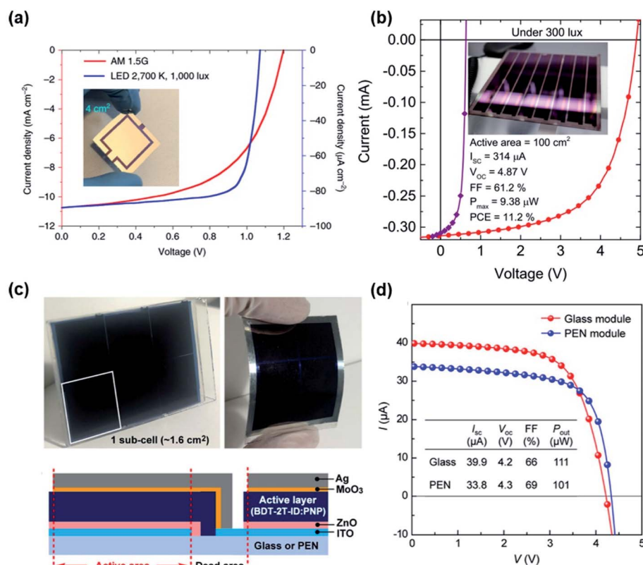
Fig. 2 (a) J–V characteristics of an OPV device with a 4.0 cm²-large area under 1 sun and an LED illumination. Inset: a photograph of the 4 cm² device. Reproduced with ref. 17 with permission from Springer Nature. (b) J–V characteristics of an 8-pixel module OPV device (red) with a total active area of 100 cm² and a pixel (purple), respectively under FL at 300 lx. Inset: a photograph taken of this module. Reproduced with ref. 23 with permission from AIP Publishing. (c) Photographs, schematic and (d) J–V characteristics of 6 series-connected devices fabricated on a glass substrate and a flexible substrate. Reproduced with ref. 38 with permission from the American Chemical Society.
