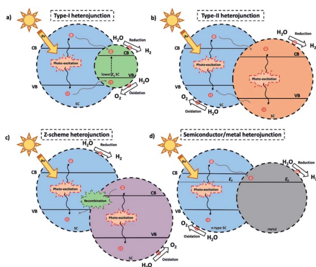
Fig. 18 Scheme of different heterojunctions based on a semiconductor heterointerface with another semiconductor: (a) Type-I, (b) Type-II, and (c) Z-scheme. (d) n-type SC interfaced with a metal ( E_F is the Fermi level), serving as the e^- sink. In all cases, CN serves as one SC (blue) and upon photoexcitation the electrons from its VB and holes from its CB may migrate according to the band alignment. On the surface, electrons may perform a reduction reaction while holes perform an oxidation one.
