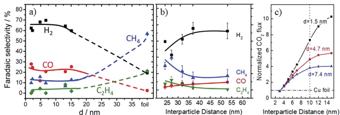
Fig. 7 (a) The faradaic efficiency of reaction products during EC CO 2 reduction on Cu nanoparticles. (b) The faradaic efficiency as a function of interparticle distances over 4.7 nm Cu nanoparticles. (c) CO 2 flux obtained for Cu nanoparticles with different sizes and interparticle distances based on diffusion equations. Experimental conditions: 0.1 M KHCO 3 , -1.1 V vs. RHE, 30 sccm CO 2 . Reproduced from ref. 65 for (a) and ref. 119 for (b) and (c), with permission from the American Chemical Society, 2014 and 2016.
