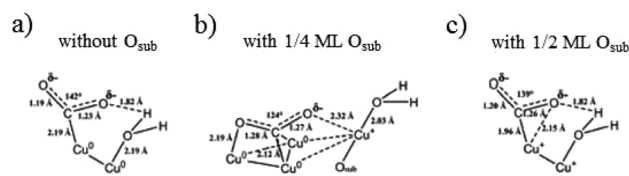
Fig. 15 Predicted structures for chemisorbed-CO 2 with H 2 O on Cu(111) with different levels of subsurface oxide O sub : (a) 0 ML, (b) 1/4 ML and (c) 1/2 ML O sub . Reproduced from ref. 96.
