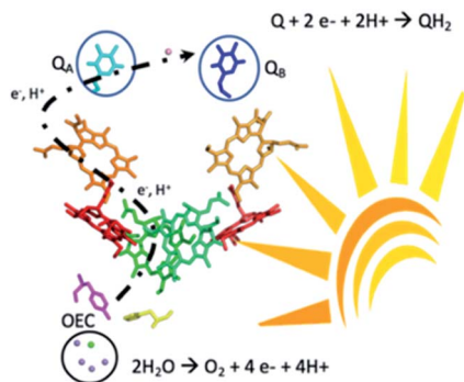
Scheme 1 Map of the main cofactors of water photo-oxidation and reactions for water oxidation at the oxygen evolving complex (OEC) and reduction of quinones Q_A and Q_B under sunlight irradiation.
