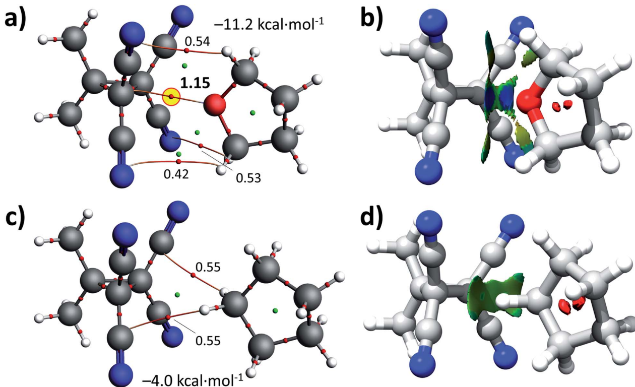
Fig. 3 Geometry optimized structures (B3LYP-D3/def2-TZVP) and 'atoms-in-molecules' analysis of [1 \cdots \text{THF}] (a, see also Fig. 2) and [1 \cdots \text{cyclopentane}] (c, obtained after in silico \text{O} \rightarrow \text{CH}_2 mutation and optimization). The bond densities of the intermolecular bond critical points are represented by small red spheres ( \rho in a.u. \times 100 ). (b) and (d) show a non-covalent interactions (NCI) analysis using NCIPLOT. Isolevel = 0.3 and regions in blue are mainly electrostatic interactions, in green are van der Waals dispersive forces and repulsions are in red.
