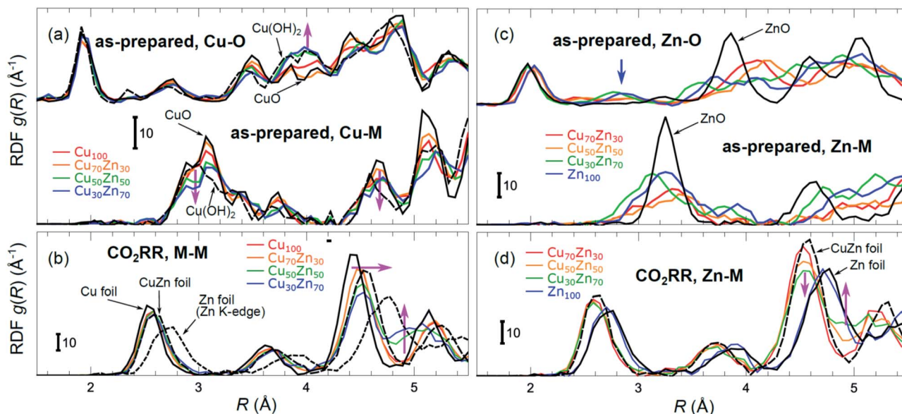
Fig. 5 Cu–O and Cu–M ( \text{M} = \text{Cu} or \text{Zn} ) RDFs extracted by NN from experimental Cu K-edge EXAFS data (see Fig. 4(a) and S4(a)†) for \text{Cu}_{100} , \text{Cu}_{70}\text{Zn}_{30} , \text{Cu}_{50}\text{Zn}_{50} and \text{Cu}_{30}\text{Zn}_{70} NPs in their as prepared state (a) as well as in their final state after 1–7 hours under \text{CO}_2\text{RR} conditions (b). Zn–O and Zn–M RDFs extracted by NN from experimental Zn K-edge EXAFS data (see Fig. 4(b) and S4(b)†) for \text{Cu}_{70}\text{Zn}_{30} , \text{Cu}_{50}\text{Zn}_{50} , \text{Cu}_{30}\text{Zn}_{70} and \text{Zn}_{100} NPs in their as-prepared state (c) as well as in their final state after 1–7 hours under \text{CO}_2\text{RR} conditions (d). Data extracted from Cu K-edge EXAFS for reference compounds (Cu foil, CuZn brass foil, CuO and \text{Cu}(\text{OH})_2 ), as well as Zn–Zn RDF, extracted from Zn K-edge EXAFS for a Zn foil are also shown for comparison in (a) and (b). Zn–O and Zn–Zn RDFs extracted by the NN from experimental Zn K-edge EXAFS for reference compounds (Zn foil, CuZn brass foil and ZnO) are shown in (c) and (d). RDFs are shifted vertically for clarity.
