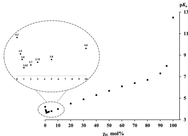
Fig. 1 \text{pK}_a values of \text{PhCH}(\text{CN})_2 versus the molar fractions \chi_{\text{IL}} of [\text{Bmim}][\text{NTf}_2] in [\text{Bmim}][\text{NTf}_2]/\text{DMSO} mixtures.
