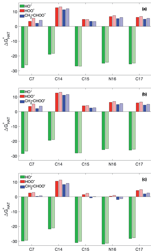
Fig. 3 \Delta G_{\text{HAT}} (kcal mol -1 ) in the gas phase (a), in benzene (b), and in water (c) for the scavenging of \text{HO}^\bullet , \text{HOO}^\bullet and \text{CH}_2=\text{CHOO}^\bullet from non-aromatic sites of selenofluoxetine. Values for fluoxetine taken from Muraro et al. 17 are showed in a lighter shade for comparison. Level of theory: (SMD)-M06-2X/6-311+G(d,p)//M06-2X/6-31G(d).
