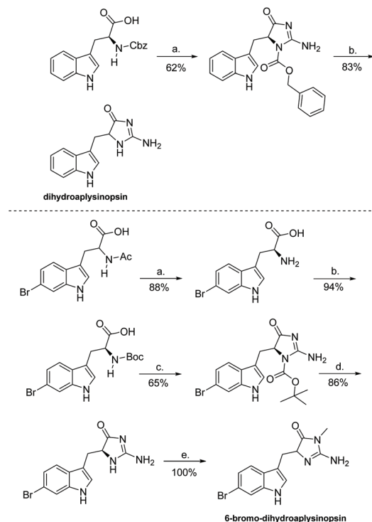
Scheme 31 Total synthesis of dihydroaplysinsopin and its 6-bromo derivative. Reagents: (a) 1. THF, DCC, NHS, 0\text{ }^\circ\text{C} , 3 h, 2. \text{NaHNCN} , \text{H}_2\text{O} , rt, 16 h, (b) \text{MeOH} , Pd/C, \text{H}_2 , rt, 1 h. Reagents: (a) Borate buffer, \text{CoCl}_2 \cdot 6\text{H}_2\text{O} , pH = 8.5, L-aminoacylase, 38\text{ }^\circ\text{C} , 48 h, (b) 1,4-dioxane, \text{H}_2\text{O} , KOH, \text{Boc}_2\text{O} , rt, 16 h, (c) 1. THF, DCC, NHS, 2 h, 2. \text{NaHNCN} , \text{H}_2\text{O} , rt, 16 h, (d) \text{MeCN} , \text{SnCl}_4 , 0\text{ }^\circ\text{C} , under Ar, 45 min, (e) \text{MeCN} , EtOH, MeI, rt, 24 h.
