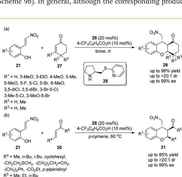
Scheme 9 Oxa-Michael/Michael cascade reaction for the synthesis of tetrahydroxanthrenones and chromans.
