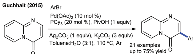
Scheme 17 C3-Arylation of pyrido[1,2- a ]pyrimidin-4-ones.
