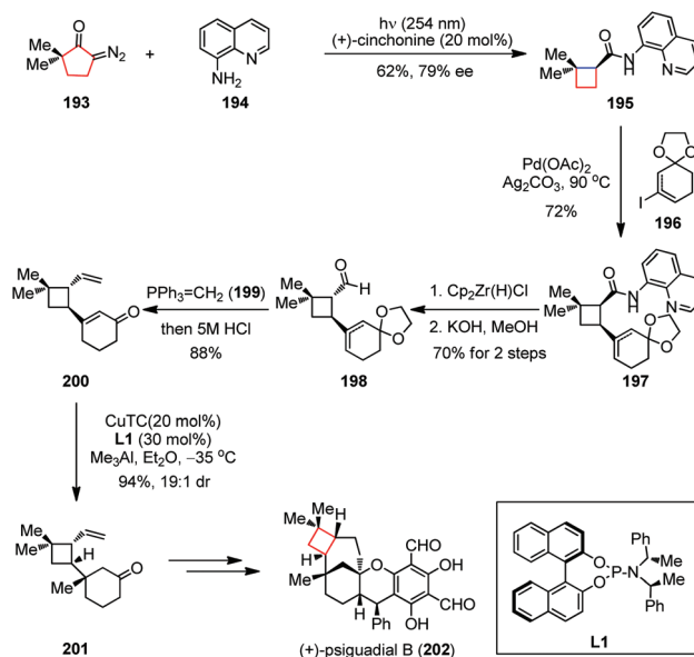
Scheme 27 Wolff rearrangement/asymmetric ketene addition cascade in the total synthesis of (+)-psguadial B.
