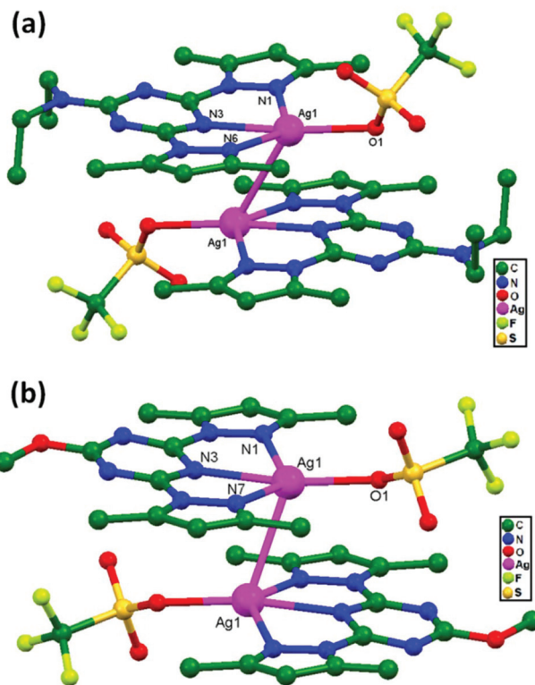
Fig. 46 The molecular structures of (a) [Ag(HL1)(OTf)] 2 , 74, and (b) [Ag(HL2)(OTf)] 2 , 75, showing ligand-unsupported argentophilic interactions.
