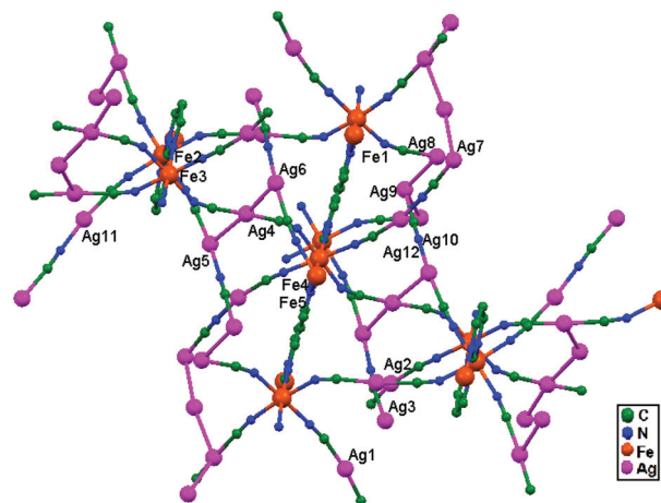
Fig. 56 The coordination environments around crystallographically inequivalent iron and silver atoms and the ligand-unsupported argentophilic interactions in \{\text{Fe}(\text{pmd})\}[\text{Ag}(\text{CN})_2][\text{Ag}_2(\text{CN})_3] , 92 .
