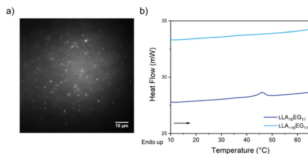
Fig. 4 (a) TIRF image of disperse \text{LA}_{\sim 16}\text{EG}_{11} upon self-assembly in water. (b) Micro-DSC traces of \text{LA}_{16}\text{EG}_{11} and \text{LA}_{\sim 16}\text{EG}_{11} at 5 \text{ mg mL}^{-1} after self-assembly in water.
